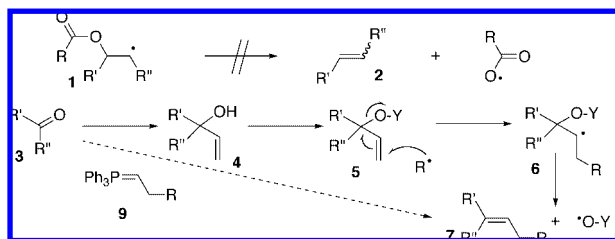
Scheme 2. Preliminary Experiments
