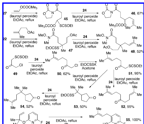
Scheme 3. Modular Construction of Substituted Olefins
